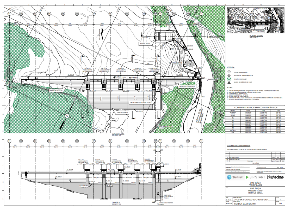
Figura 3 – Arranjo Geral da barragem – As Is
