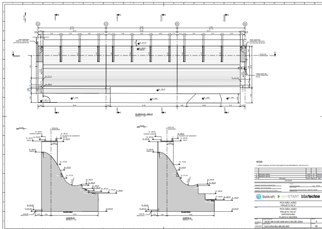
Figura 5 – Projeto As Is do vertedouro
