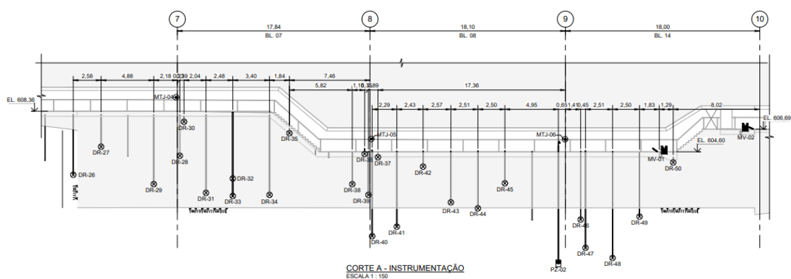
(c) Vertedouro
